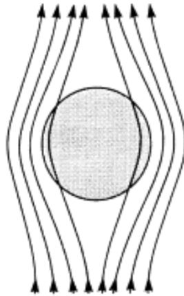
Figure 3: Magnetic field lines around the diamagnetic sphere
